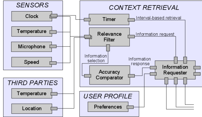
Fig. 3. Overview of the Context Retrieval component
